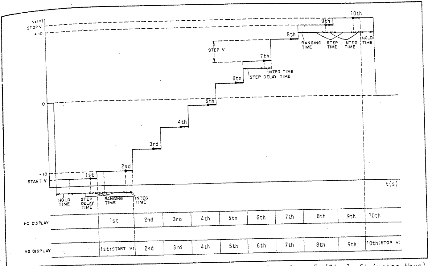
Figure 3-13. Relationship between I-V Measurement and Displays for \text{f} (Single Staircase Wave).
