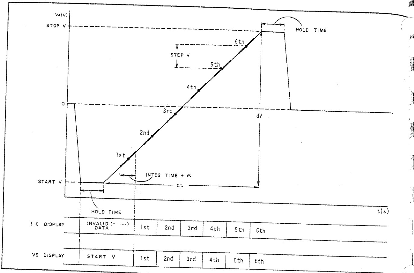
Figure 3-15. Relationship between I-V Measurement and Displays for \surd (Single Ramp Wave).
