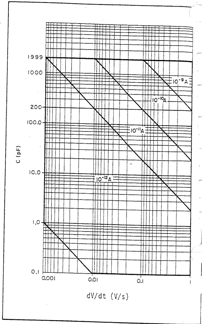
Figure 3-21. Suitable Current Measurement Ranges for C-V Measurements.
