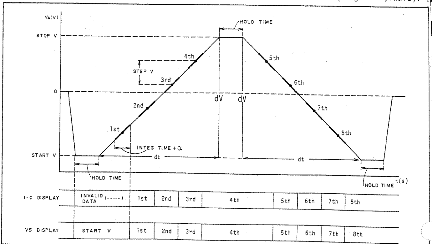
Figure 3-19. Relationship between C-V Measurement and Displays for \searrow (Double Ramp Wave).
